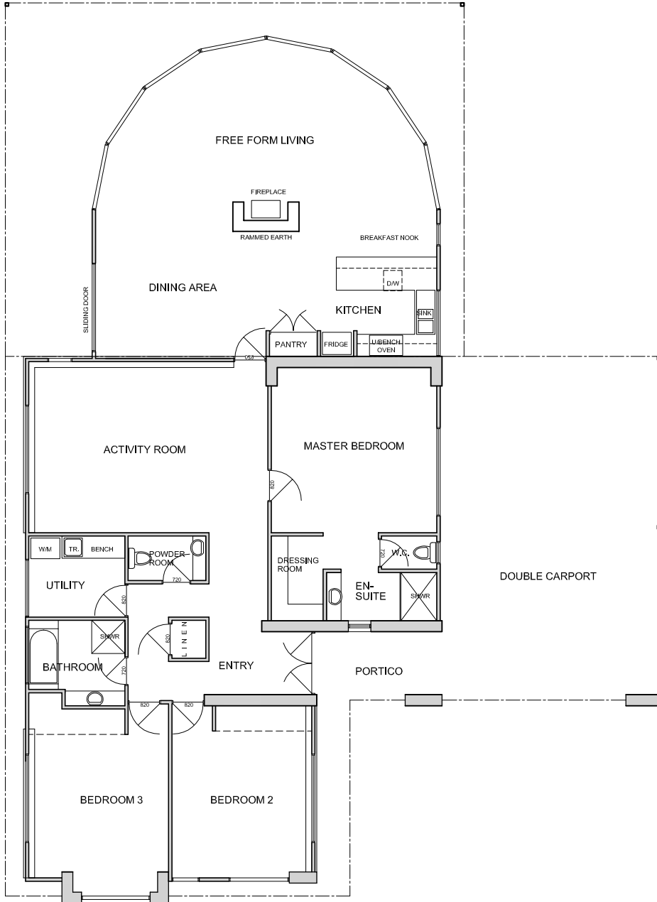
FLOOR PLAN
